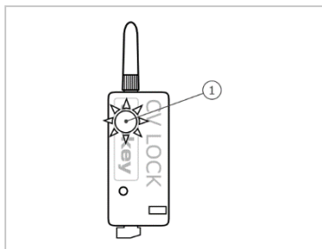
Fig. 4: Optical signals on the radio emitting module
